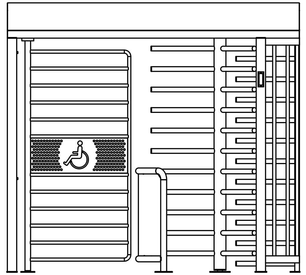
Instalation tamplate
